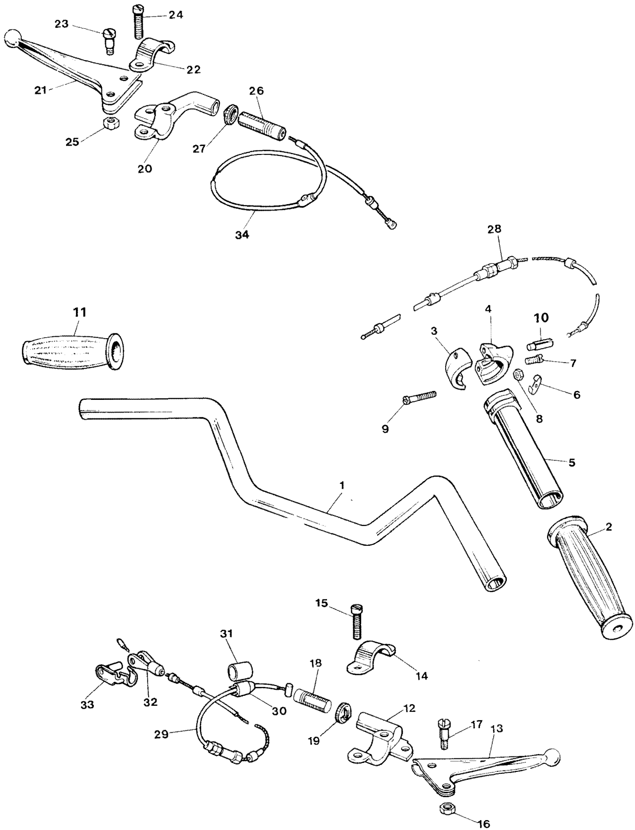
Fig. 14. HANDLEBARS, CONTROL LEVERS AND CABLES
