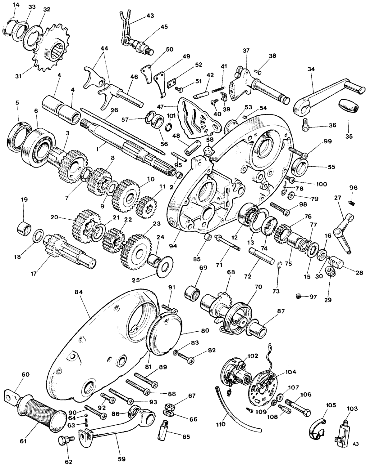
Fig. 3. GEAR CLUSTER AND TIMING COVERS
