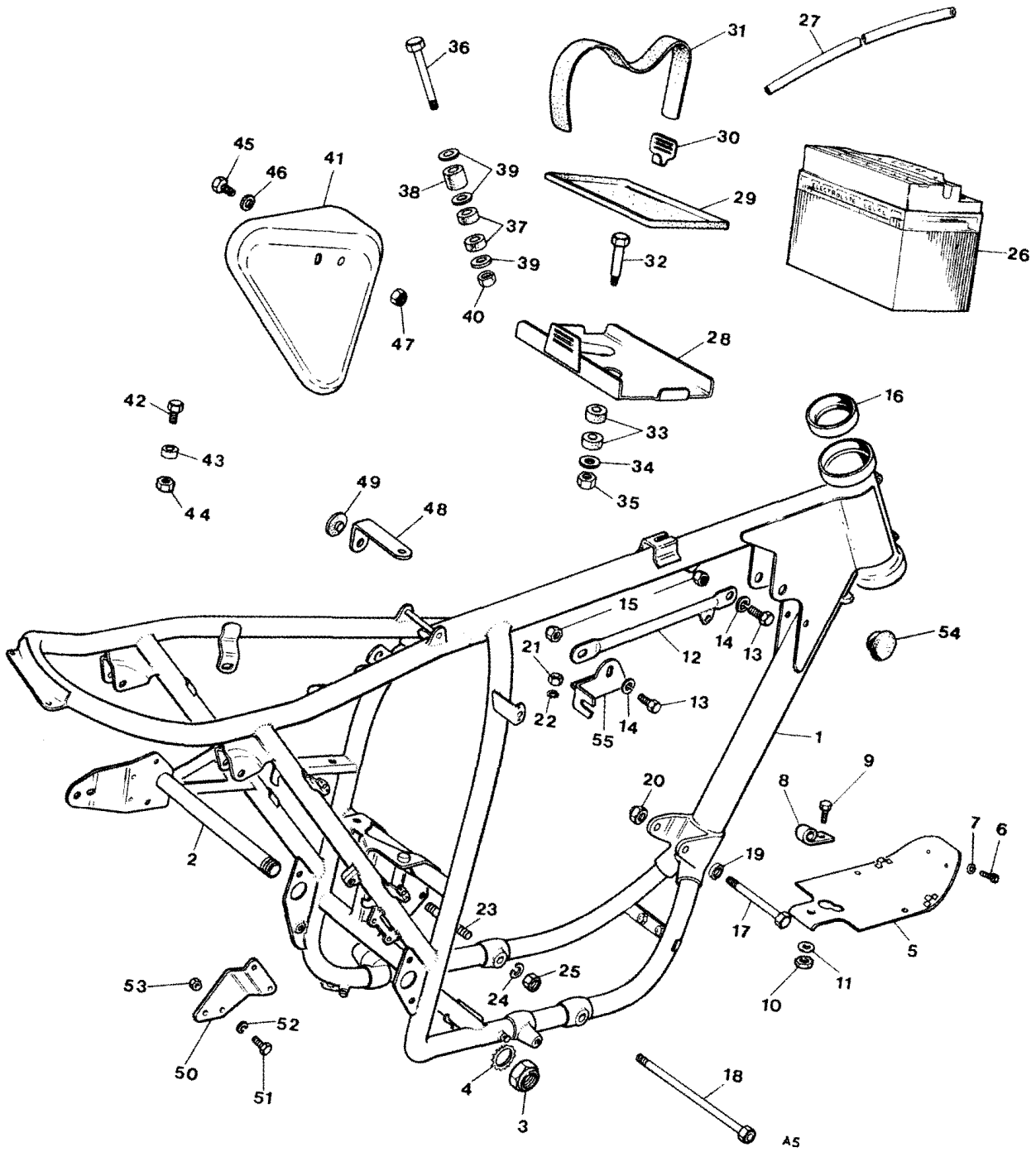
Fig. 5. FRAME COMPLETE
