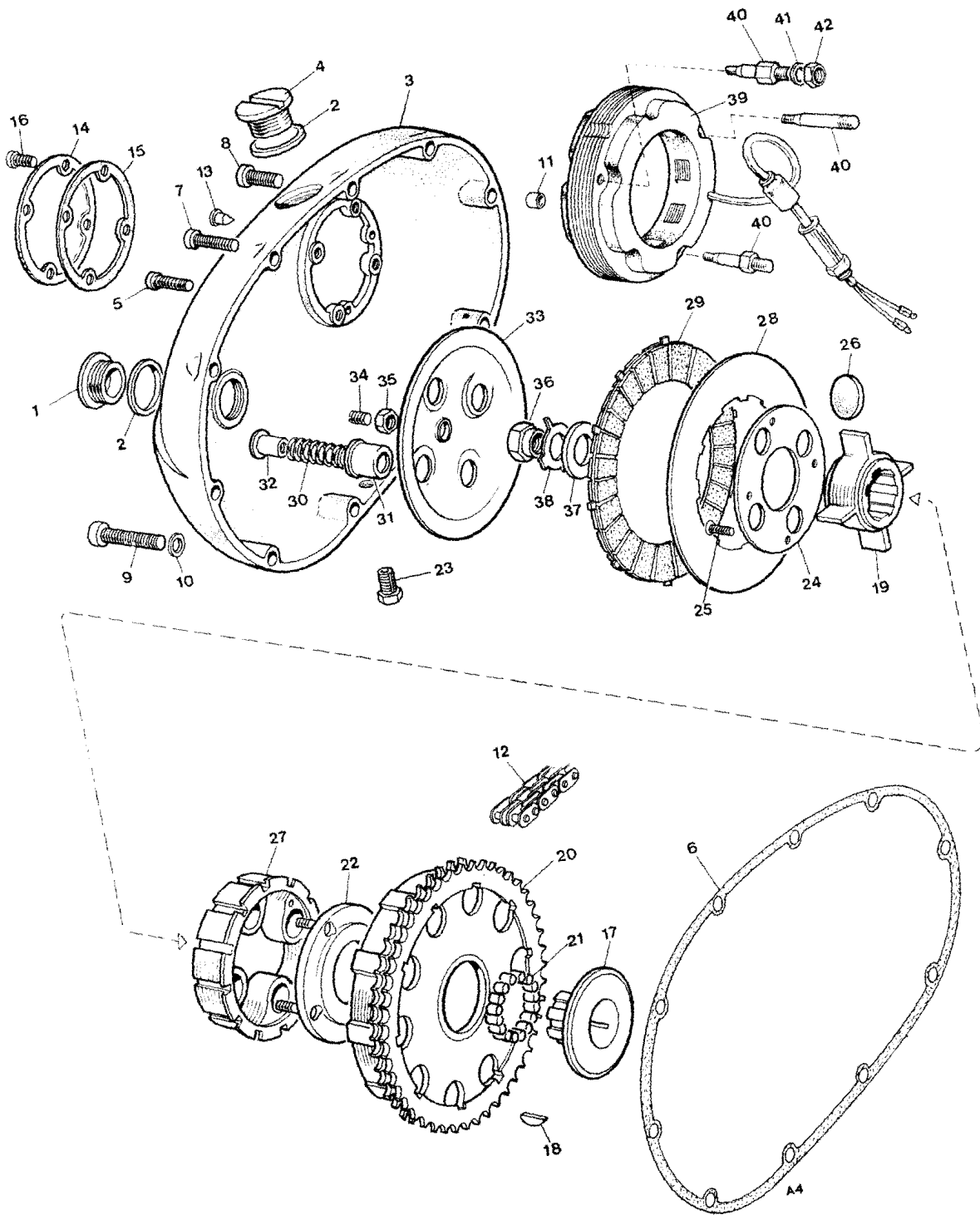
Fig. 4. CLUTCH AND PRIMARY CHAINCASE
