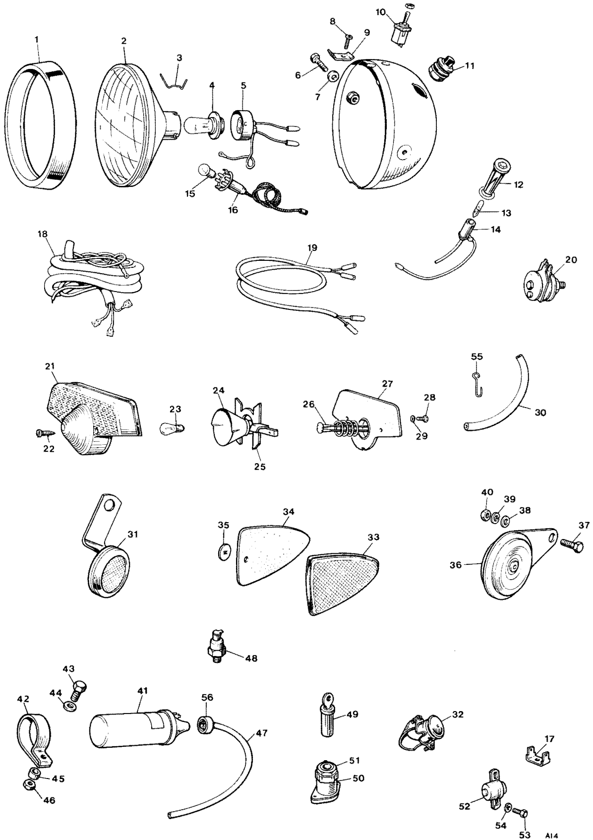
Fig. 16. ELECTRICAL EQUIPMENT
