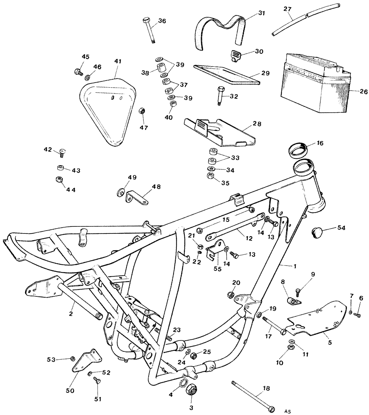
Fig. 5. FRAME COMPLETE
