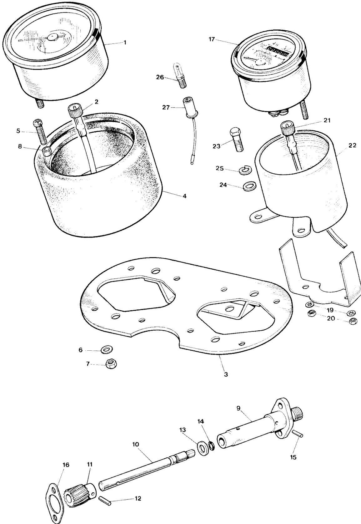
Fig. 15. SPEEDOMETER AND TACHOMETER
