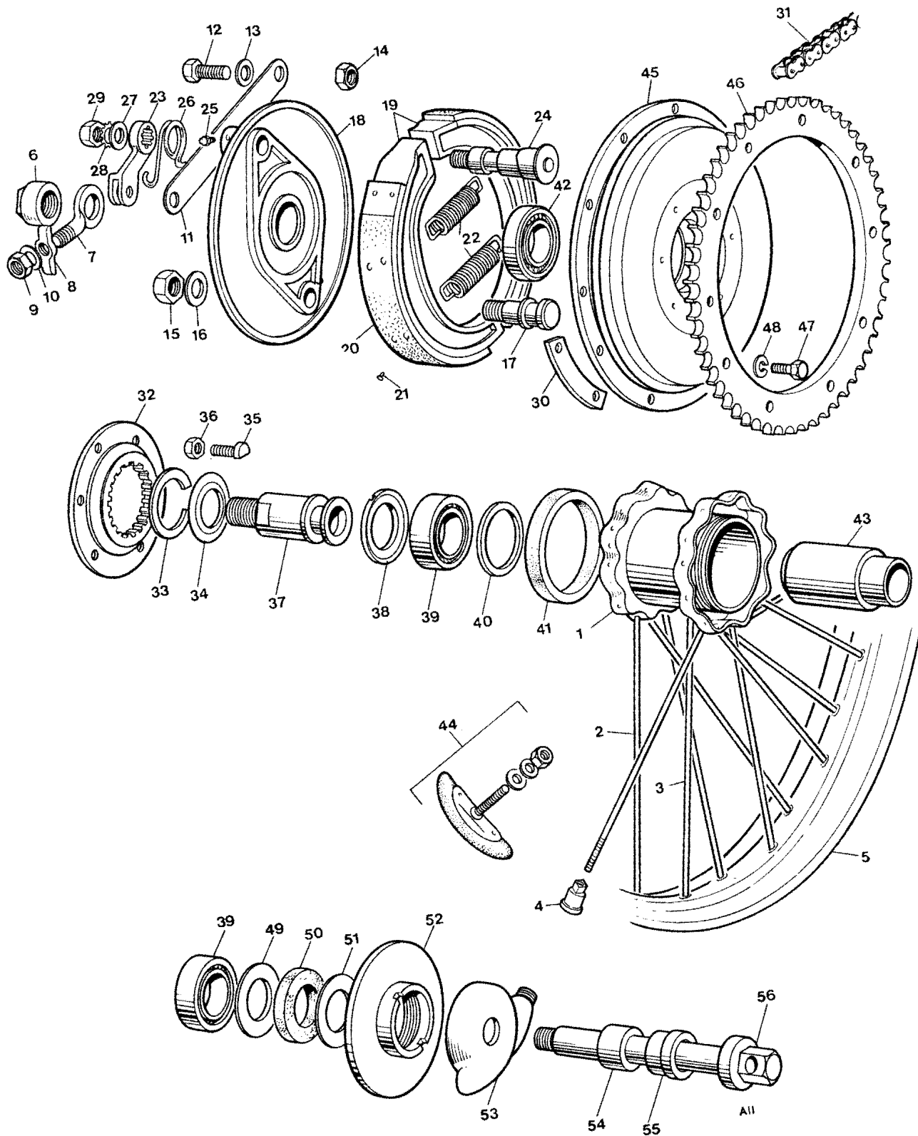
Fig. 11. REAR WHEEL
