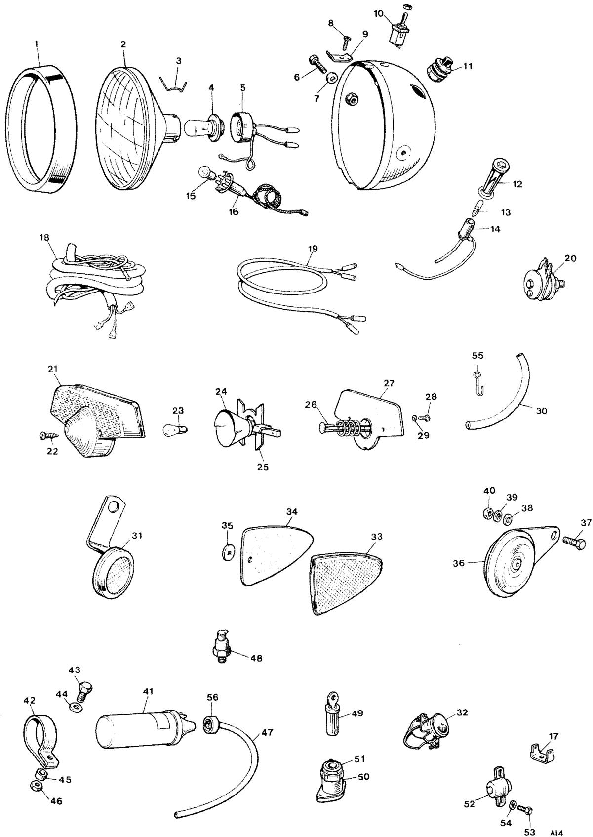
Fig. 16. ELECTRICAL EQUIPMENT
