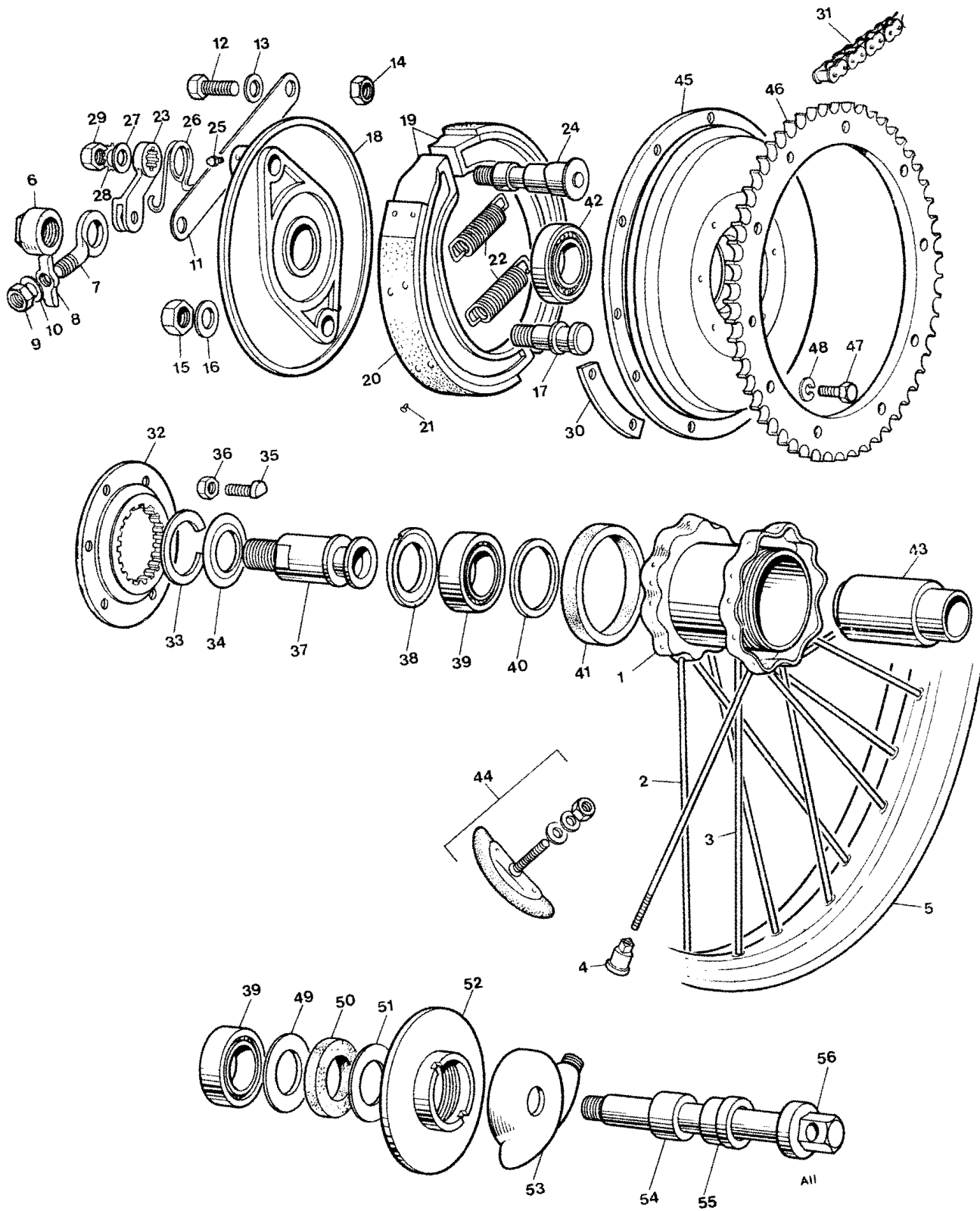
Fig. 11. REAR WHEEL
